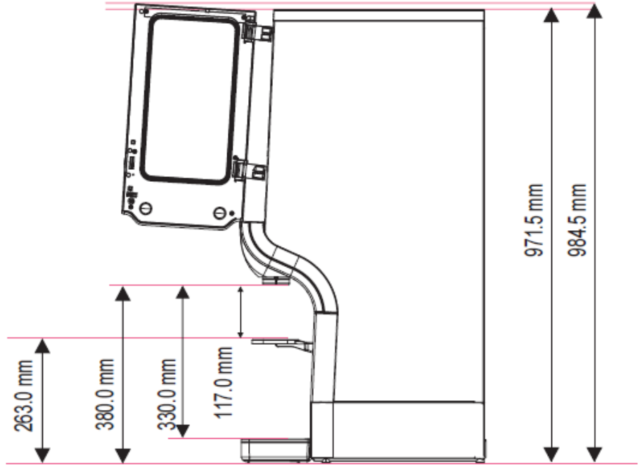
C120 NG Kit Airpot extension
